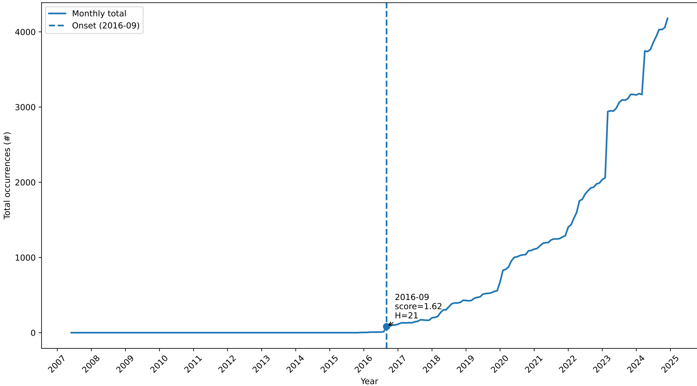
Coroutines (async and await syntax) — Onset of generalized adoption (ruptures + median)
